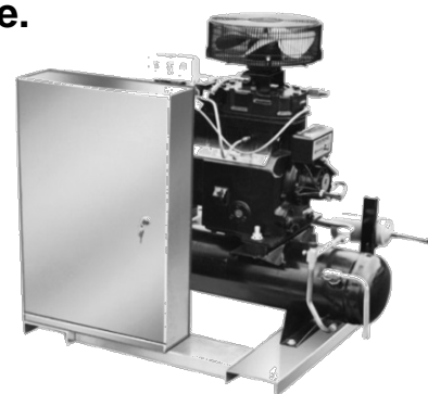
Shown with optional oversized control panel, liquid line assembly, suction line assembly and Electronic oil pressure control.
